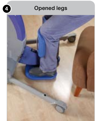
4 Opened legs For transfers, the powered chassis can be opened for optimum access.
